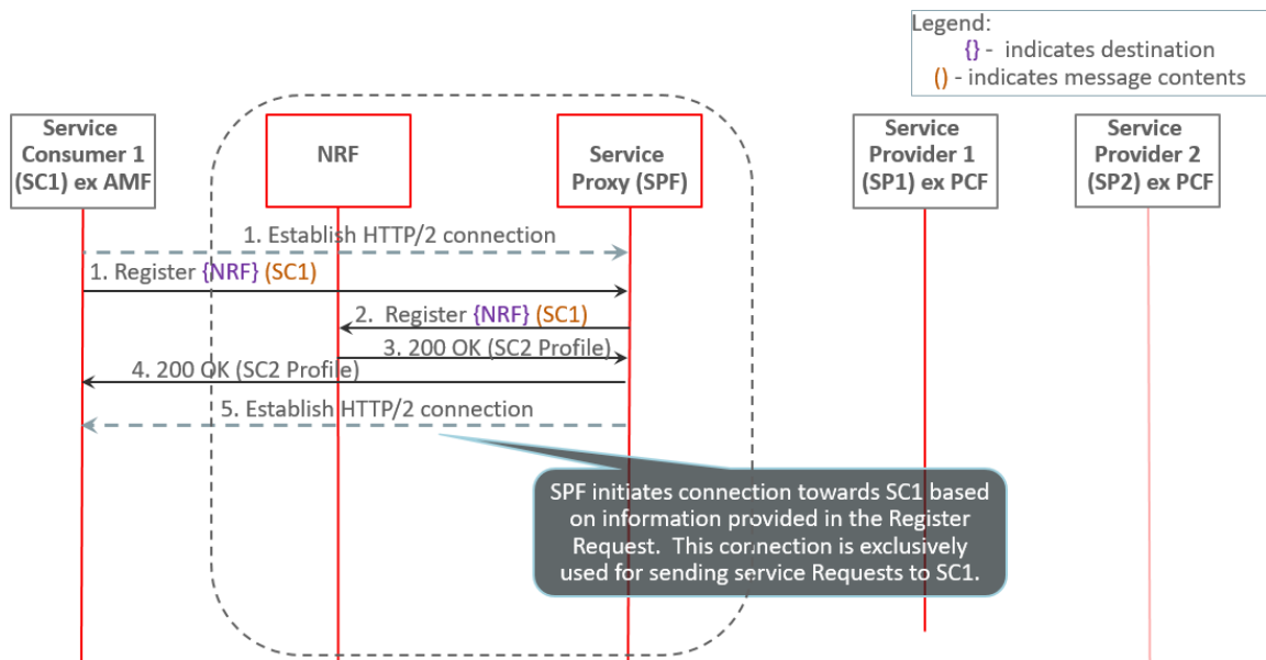
Figure 68 – NF registration call flow - Consumer
