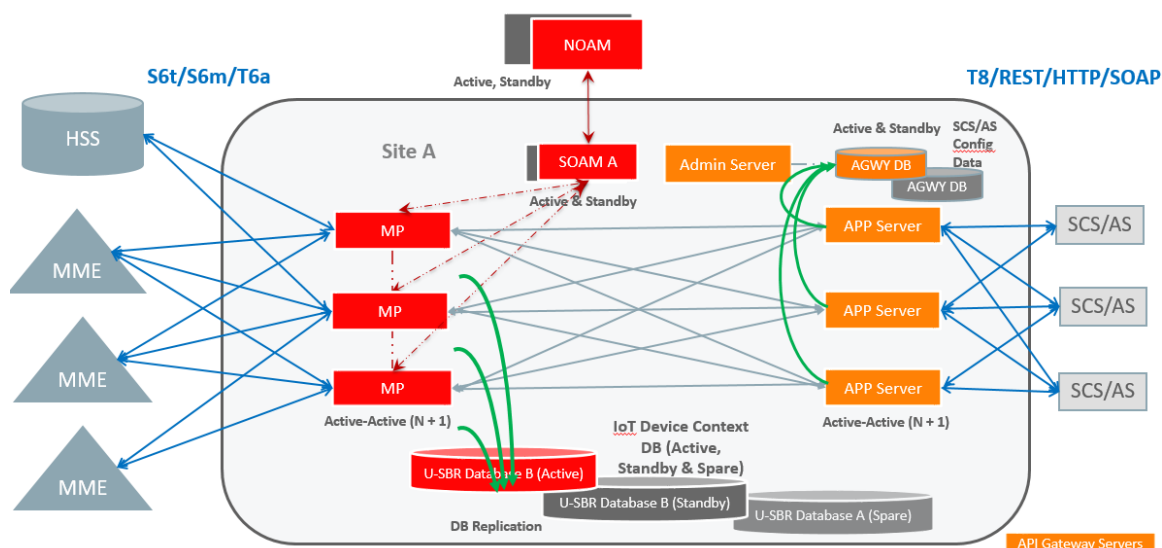
Figure 65: SCEF site architecture example
