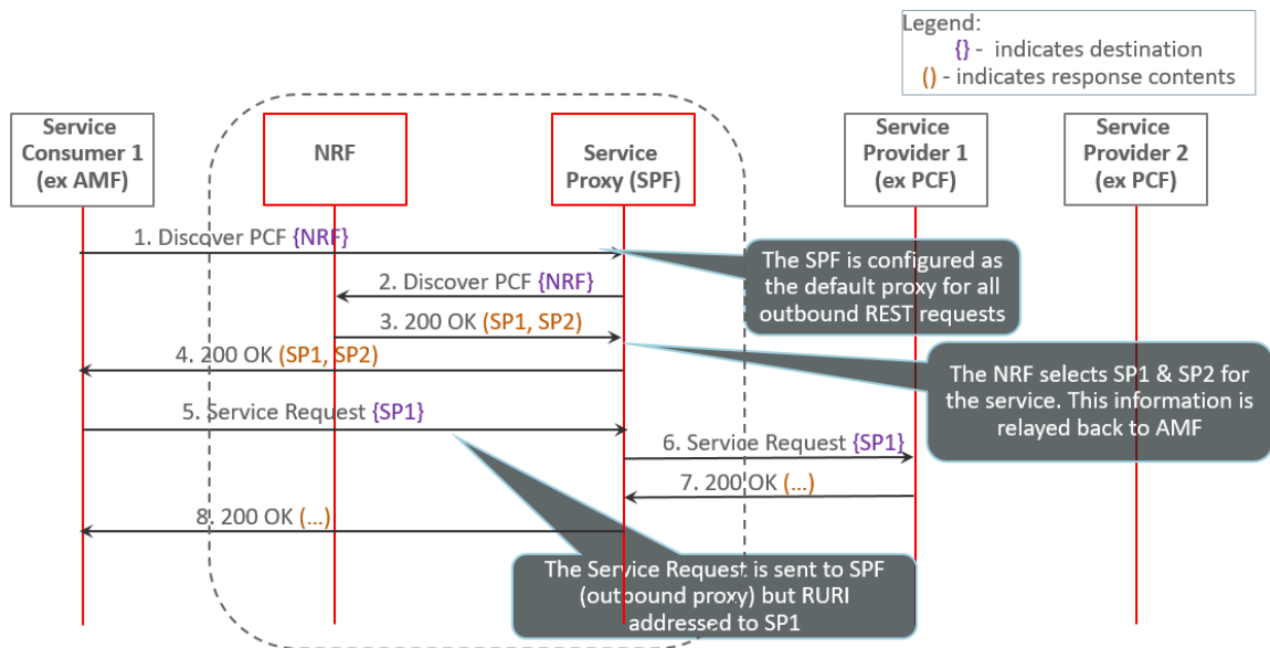
Figure 70 – Discover & Service Request Routing
