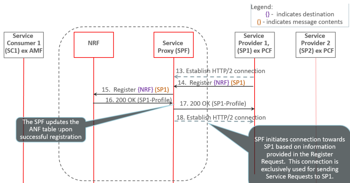
Figure 69 – NF registration call flow - Provider
