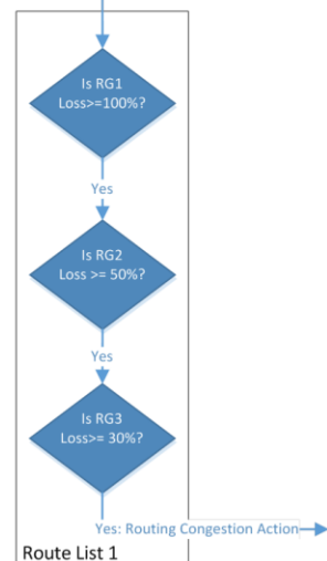
Figure 40 - Congestion-Aware Route List Logic Example 1b
