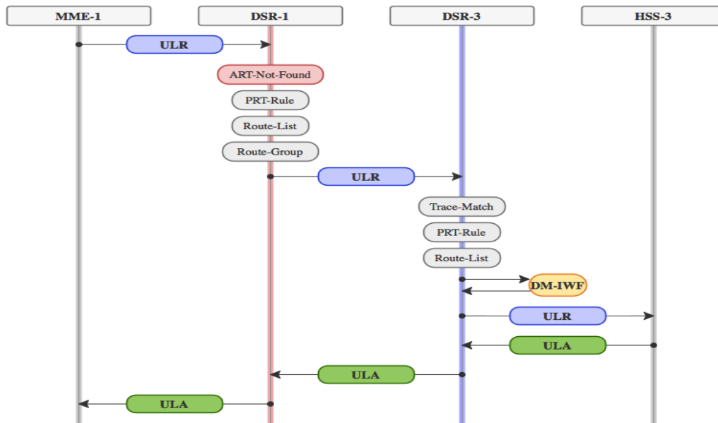
Figure 75 – Message Flow for Network Wide Trace
