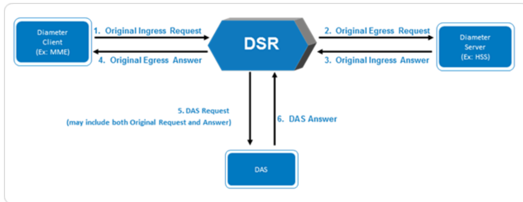
Figure 66 - Message Copy Overview
