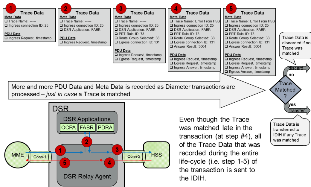
Figure 73 - IDIH Trace Data
